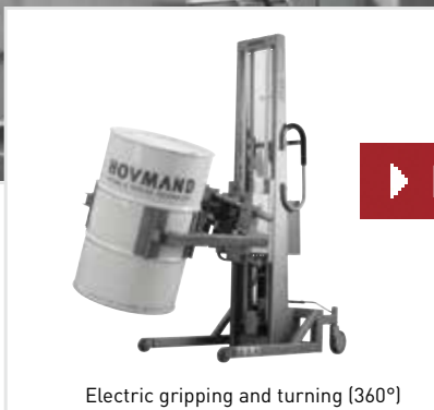
Electric gripping and turning (360°)
